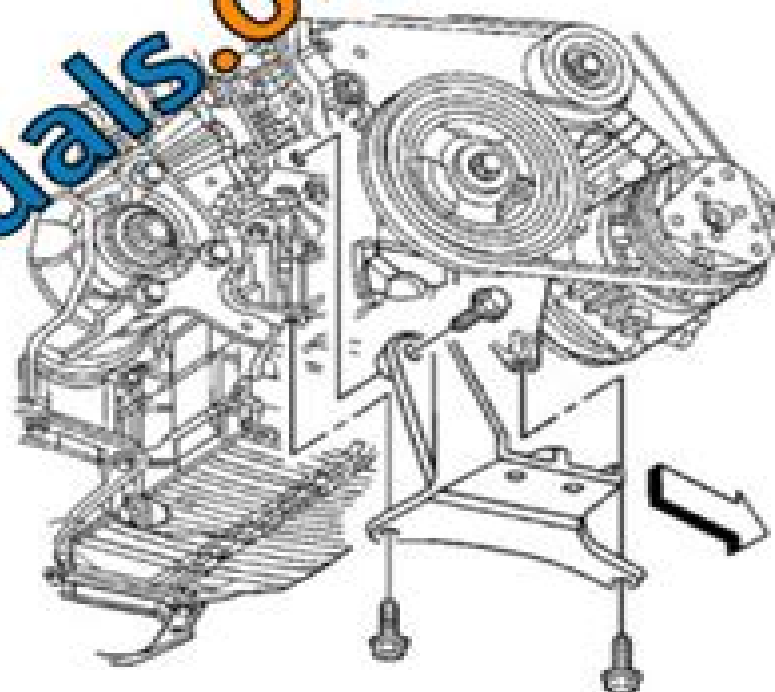
Fig. 19: View Of Engine Mount Bracket Bolts At Engine Courtesy of GENERAL MOTORS CORP.
