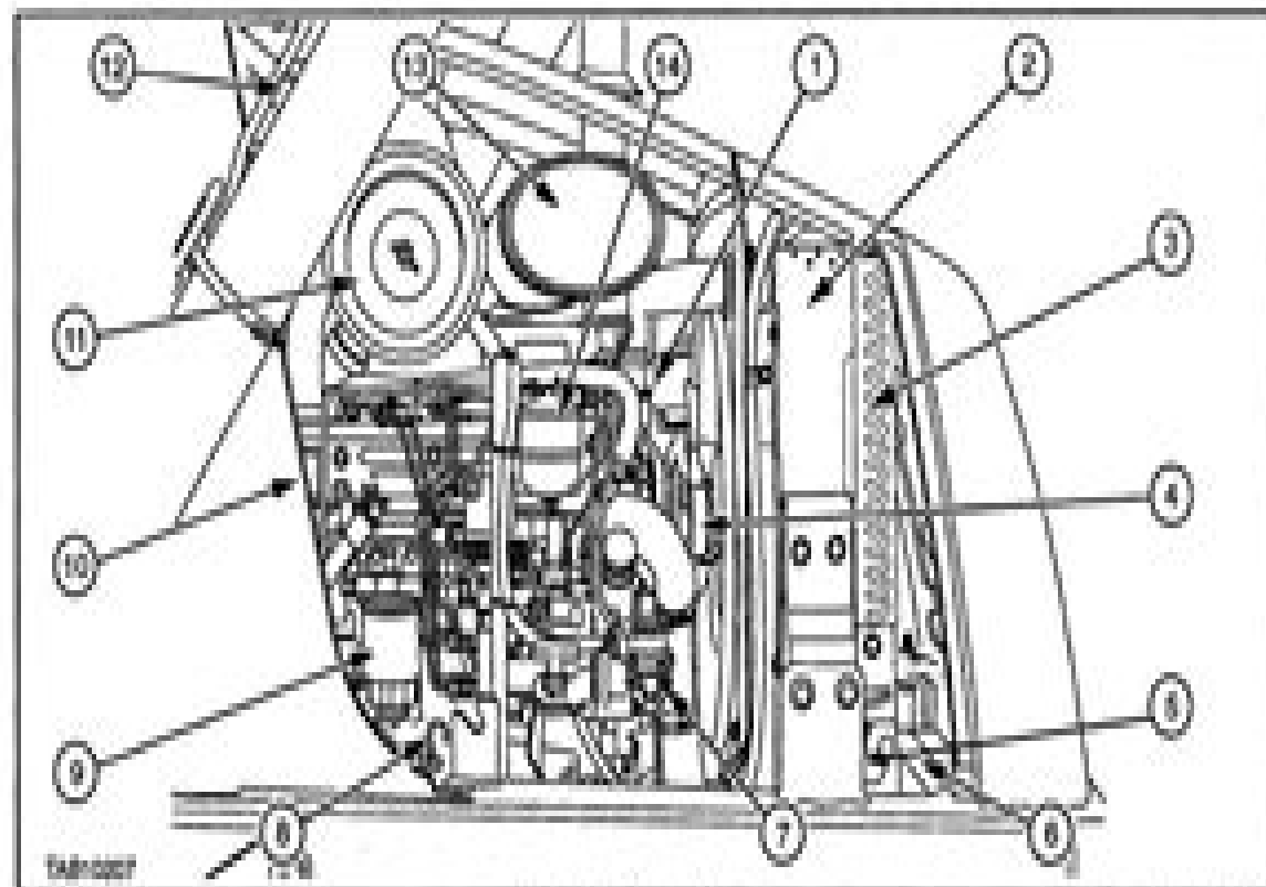
Right-Hand View of Engine
