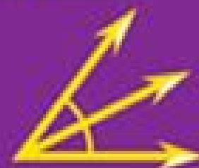
Angle Bisector
