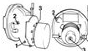
1. Lead plug 2, 3. Grease nipples Disengageable clutch
