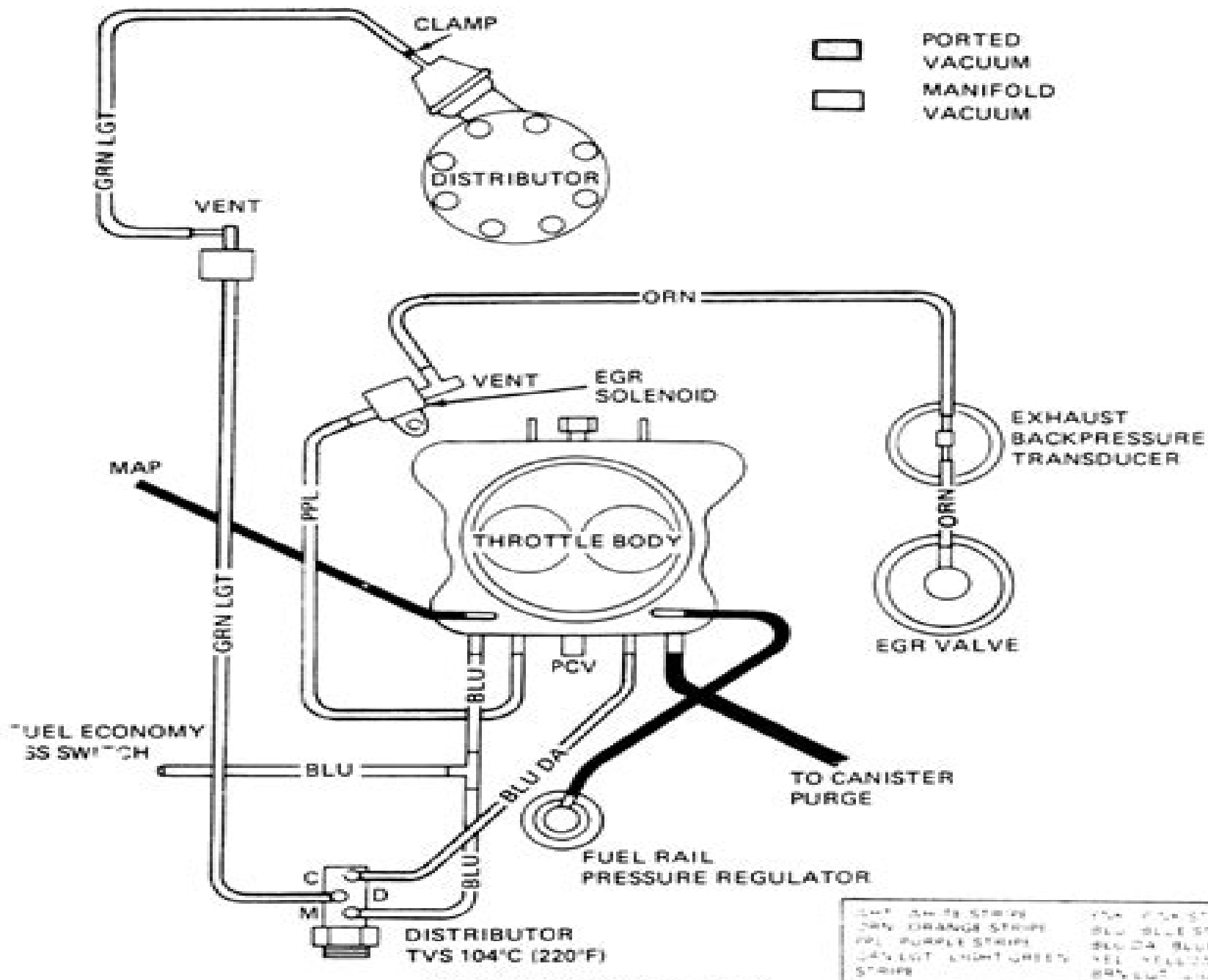
VACUUM HOSE SCHEMATIC (EMISSION SYSTEMS EXCEPT EVAP CANISTER)
