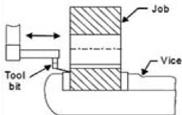
Keyway cutting
