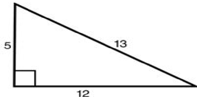
5-12-13 Triangle
