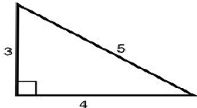
3-4-5 Triangle
