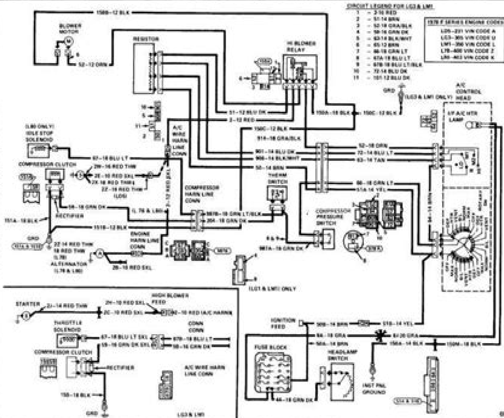
Fig. 18-4 1976 F Series C60 A/C Wiring
