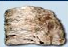
33. Barite
