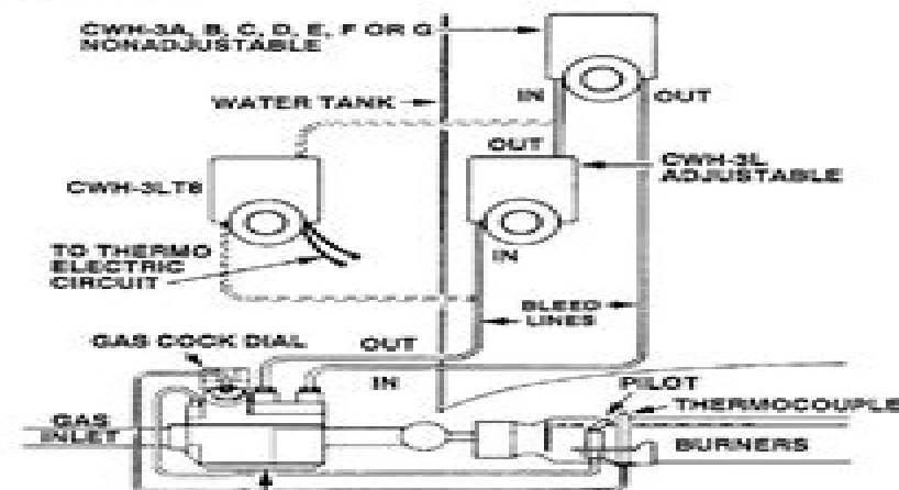
700-800 SERIES GAS VALVE
