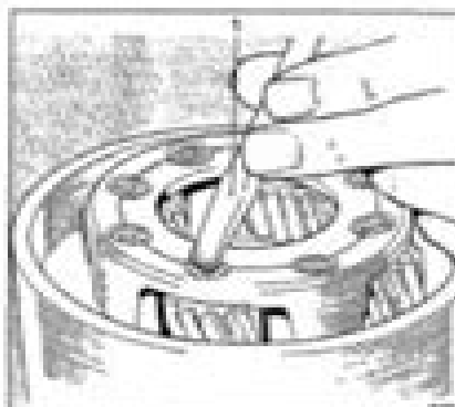
Fig. 715-14 Staking a piston pin 1. Crank
