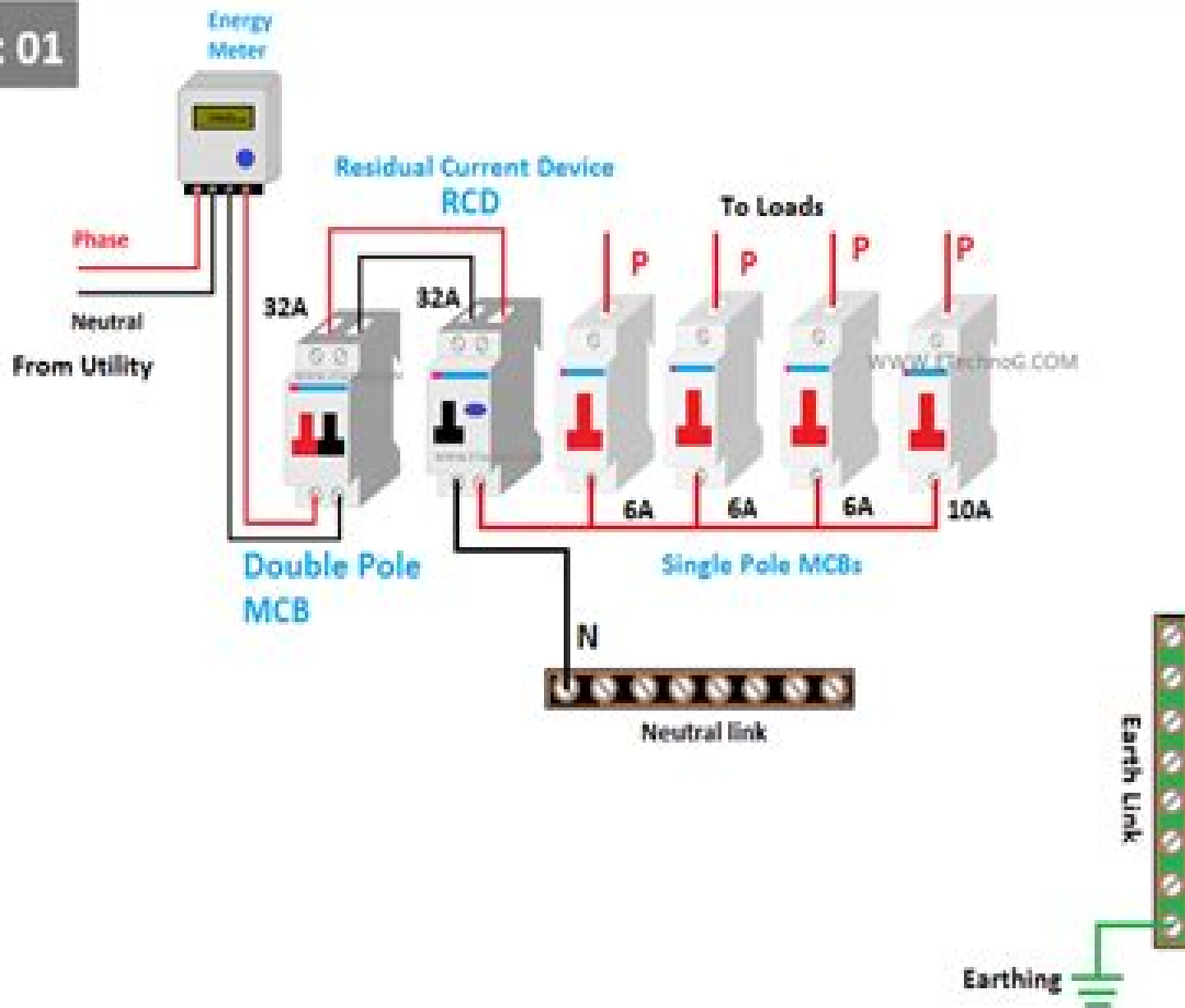
Residual Current Device(RCD) Connection & Wiring Diagram
