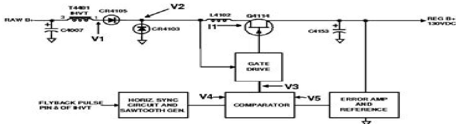
Figure 1, Main Regulator Block Diagram
