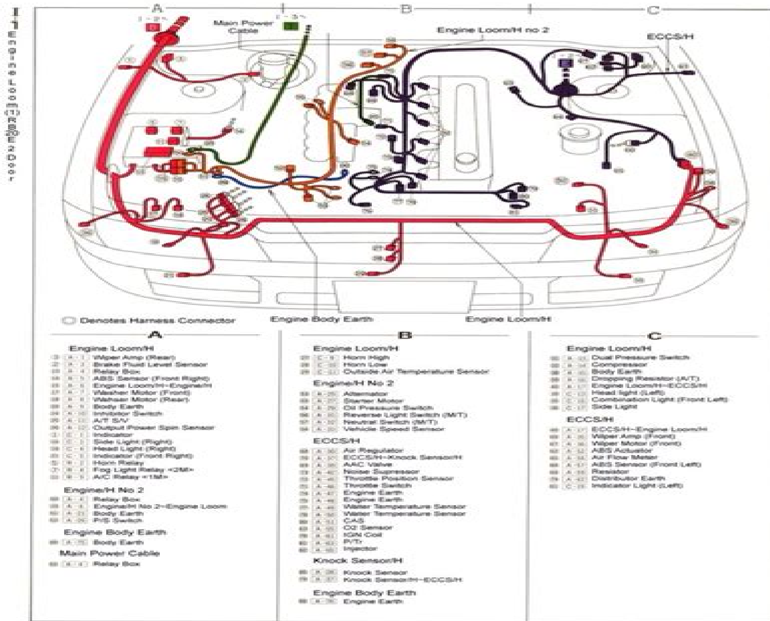
R33 Wiring Diagram
