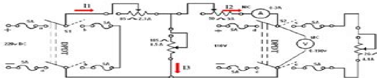
Fig. 1: Circuit diagram for verification in physical lab
