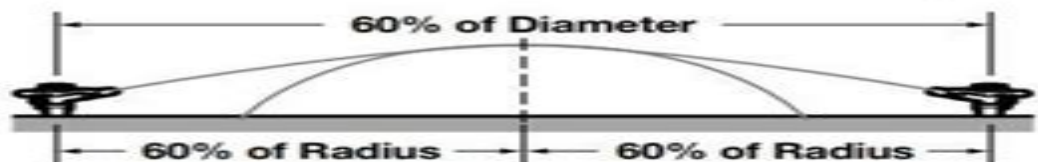
Figure 35: 60% diameter sprinkler spacing
