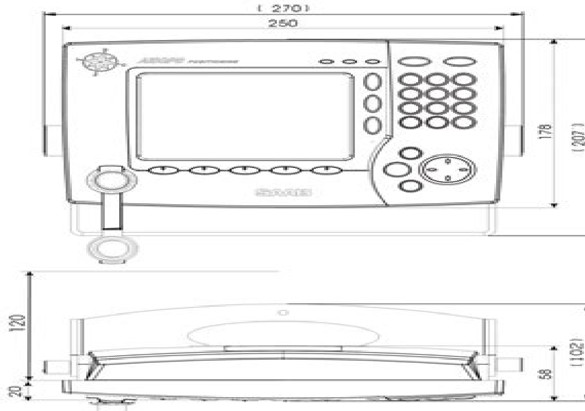
Figure 4-2: Mechanical drawing R4 Display
