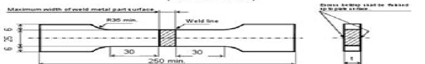
Figure 2 Tension test piece for butt welded joint of plates (No. 1 Test piece)
