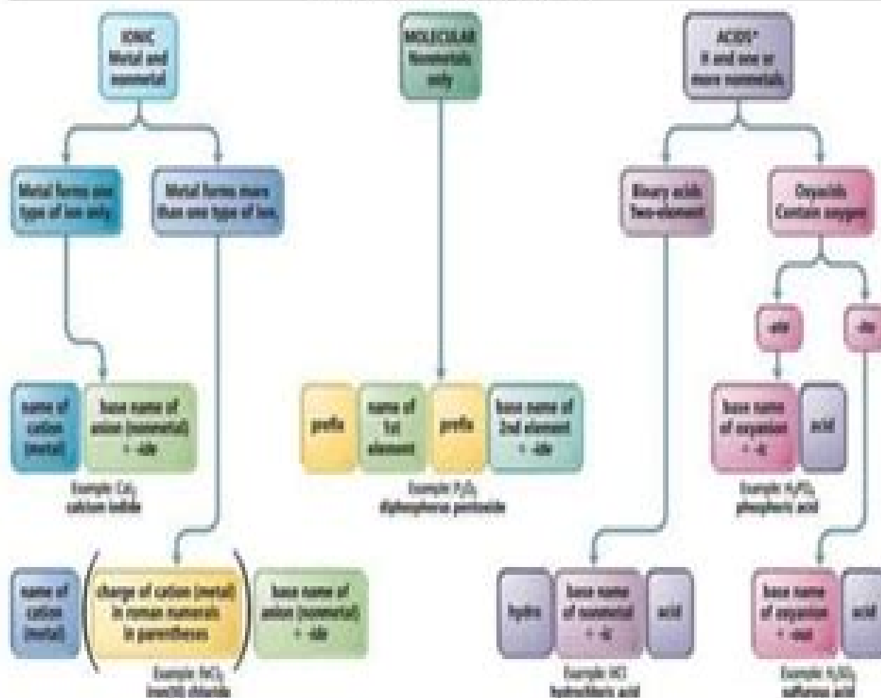
Inorganic Nomenclature Flow Chart
