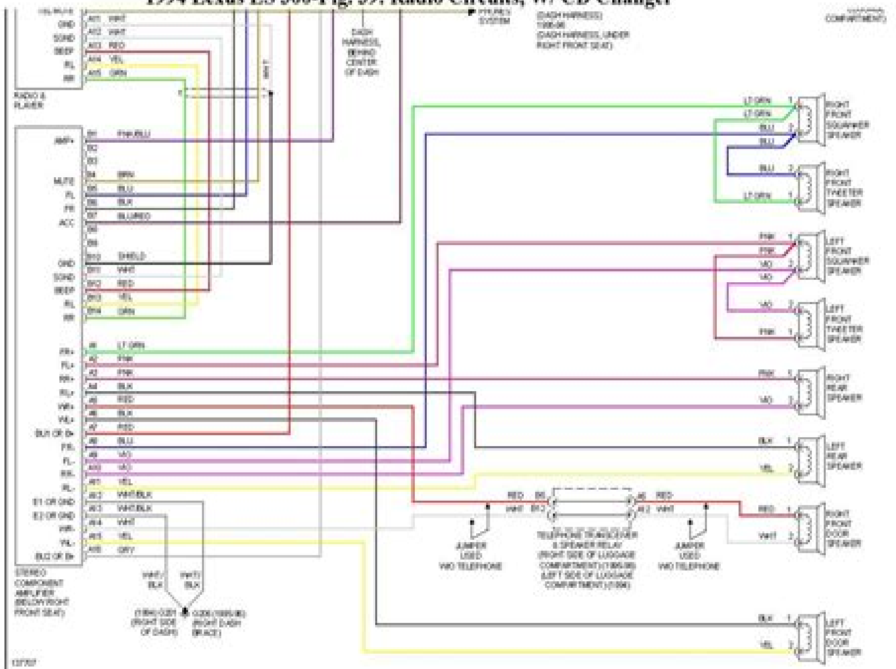
1994 Lexus ES 300-Fig. 39: Radio Circuits, W/ CD Changer
