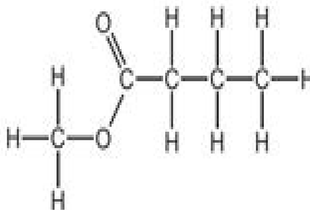
methyl butanoate
