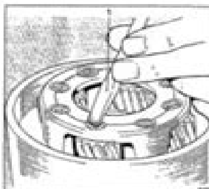
Fig. 11B-14 Staking a pin into a hole
