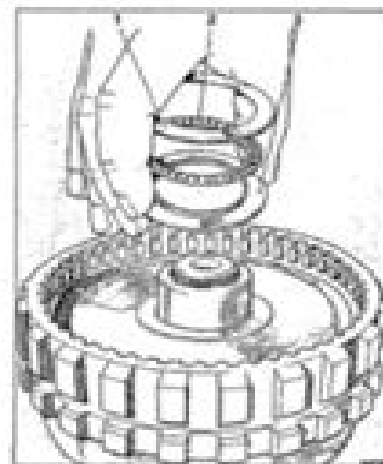
Fig. 715-16 Fitting the rear and thrust bearing to the outer face of the rear internal gear 1. Oil 2. Thrust bearing 3. Oil
