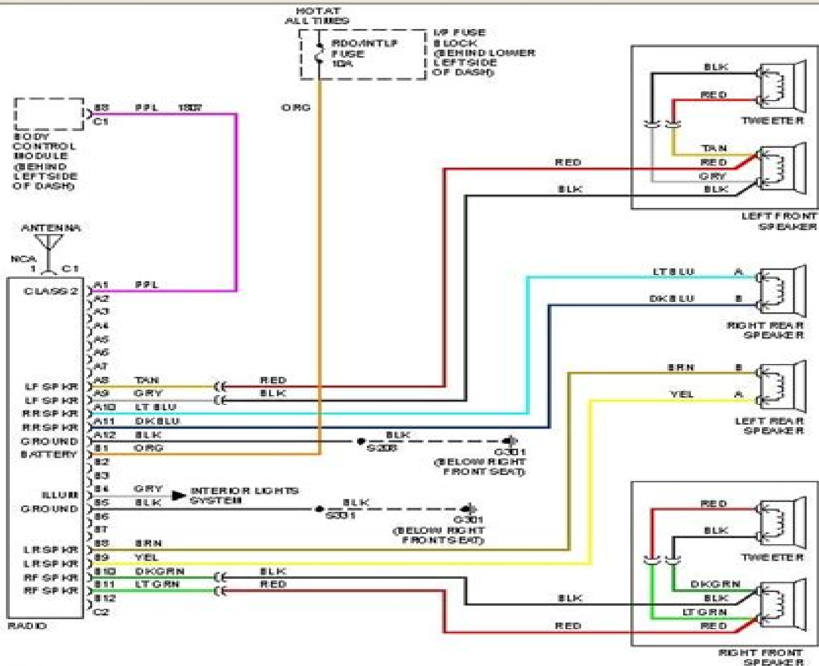
Fig. 42: Radio Circuits, W/O Amplifier
