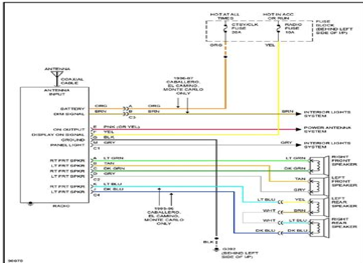
Fig. 7: Mono Radio Circuit
