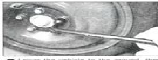
8 Lower the vehicle to the ground, then finally tighten the wheel bolts in a diagonal sequence. Note that the wheel bolts should be tightened to the specified torque at the earliest opportunity.
