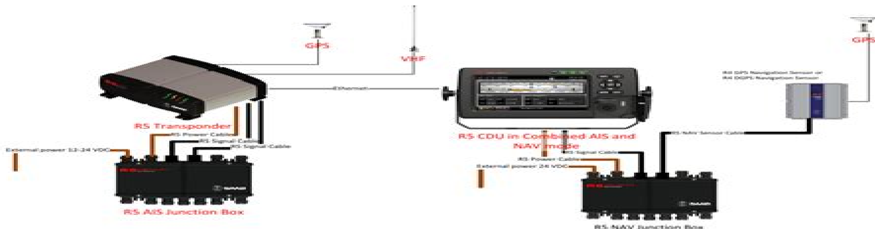
Figure 46- Combined AIS and Navigation system
