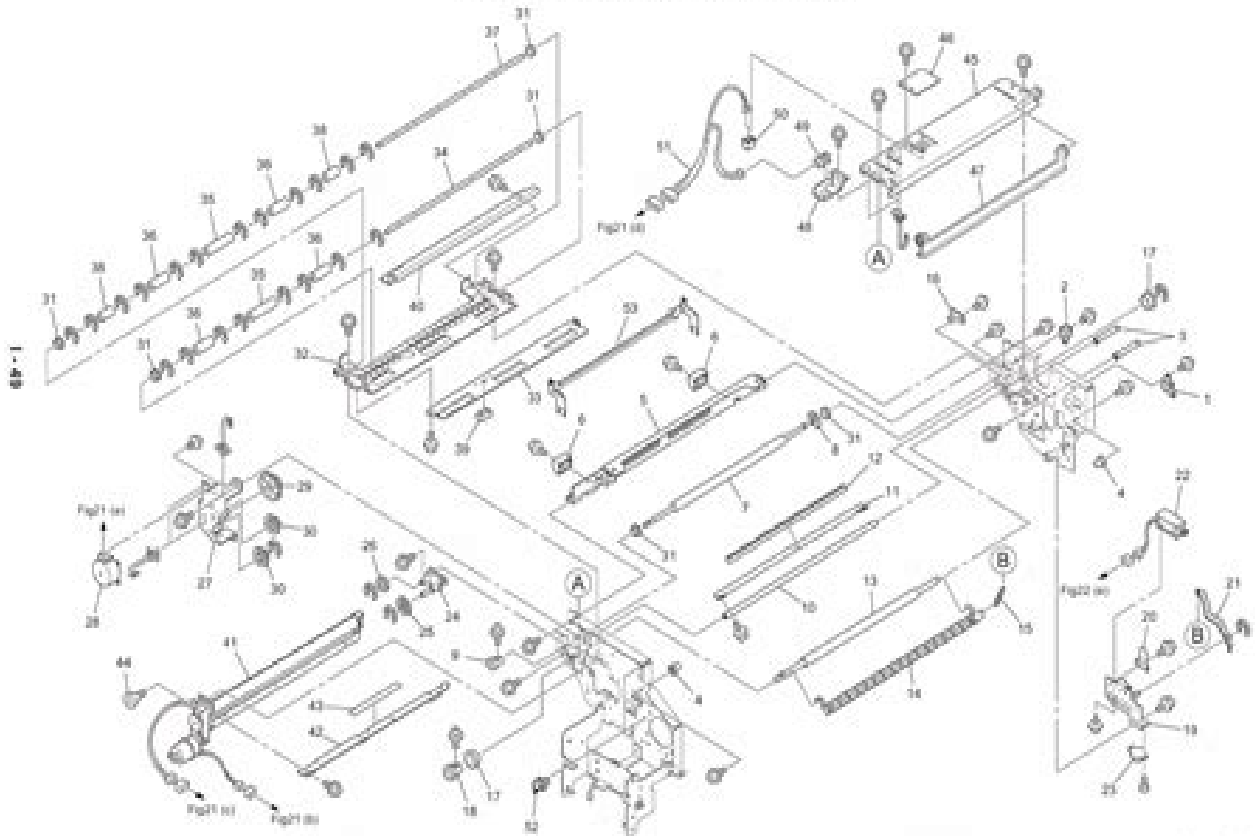
Fig24. Master-Making Area (4)
