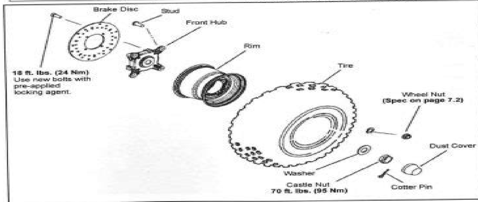
Front Hub/Wheel Exploded View
