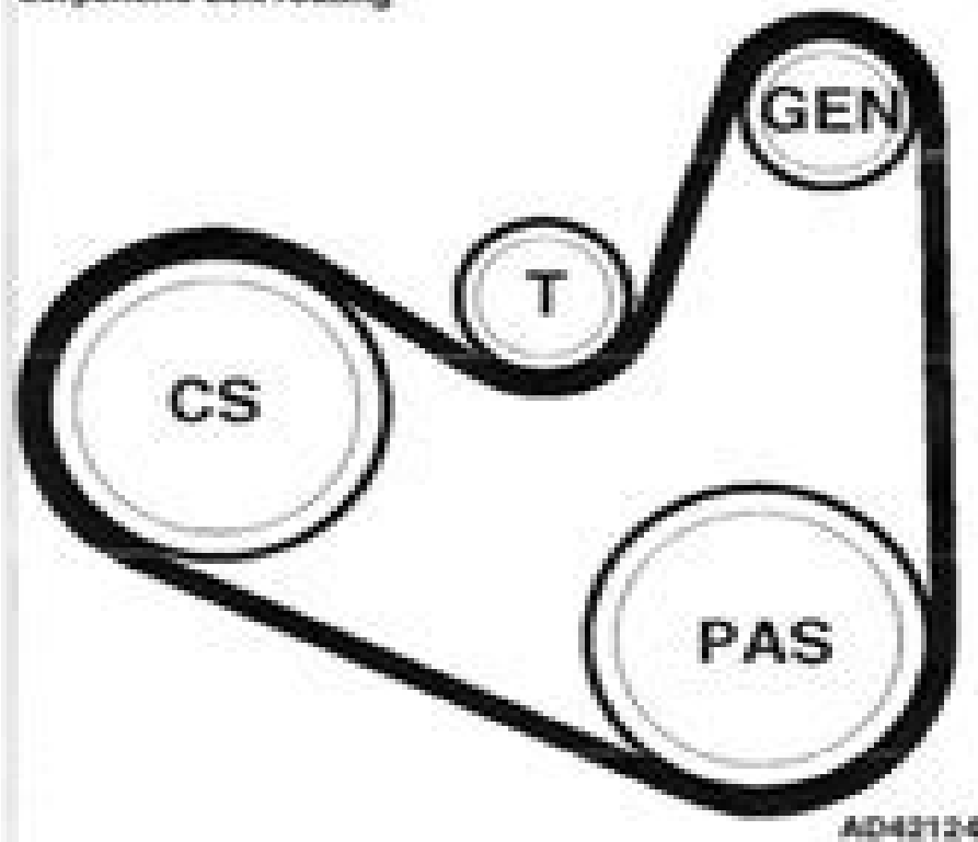
Serpentine belt routing
