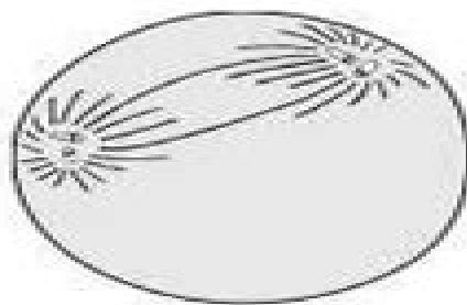
Prophase I
