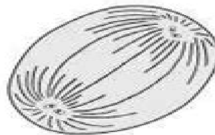
Anaphase II
