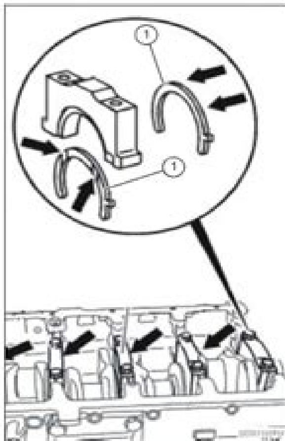
Fit bearings and thrust washers.
