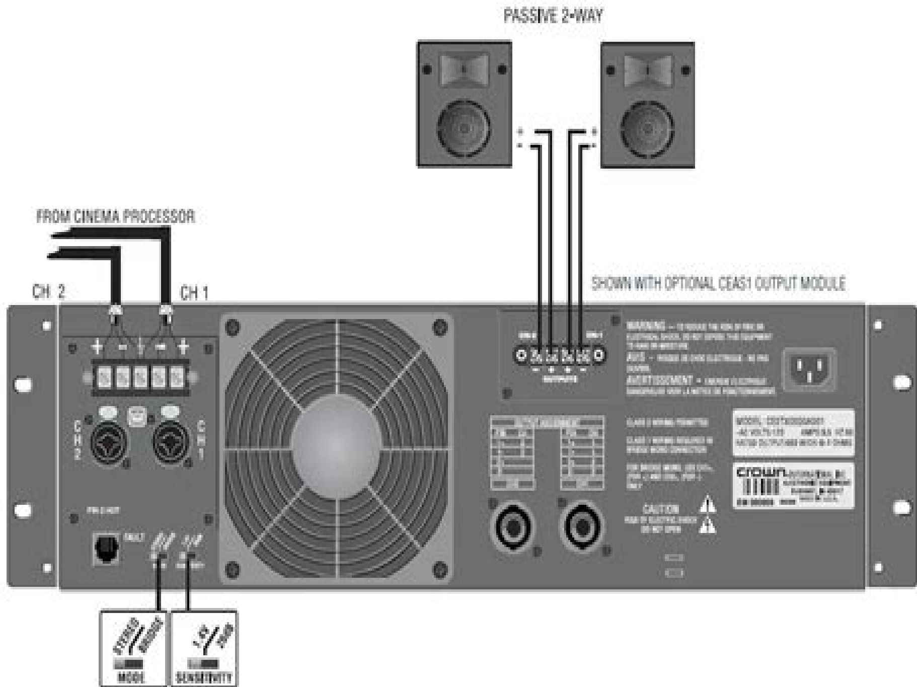
Figure 3.9 Typical System Wiring, Stereo Mode
