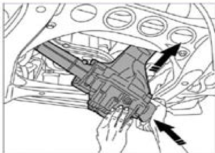
Fig. 324: Installing front-wheel final drive
