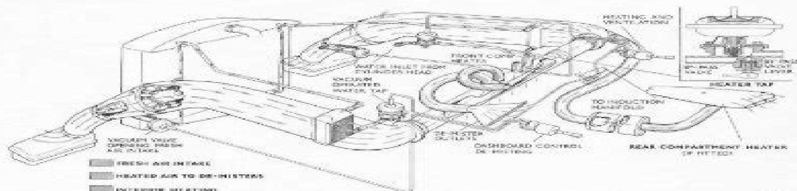
Fig. C1 Early System as fitted to early Standard S1 and early Continental S1 cars
