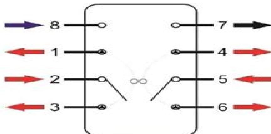
CIRCUIT DIAGRAM
