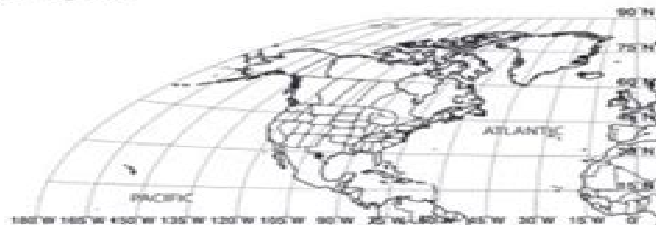
Figure 5. Northern Pacific and Atlantic ocean basins.
