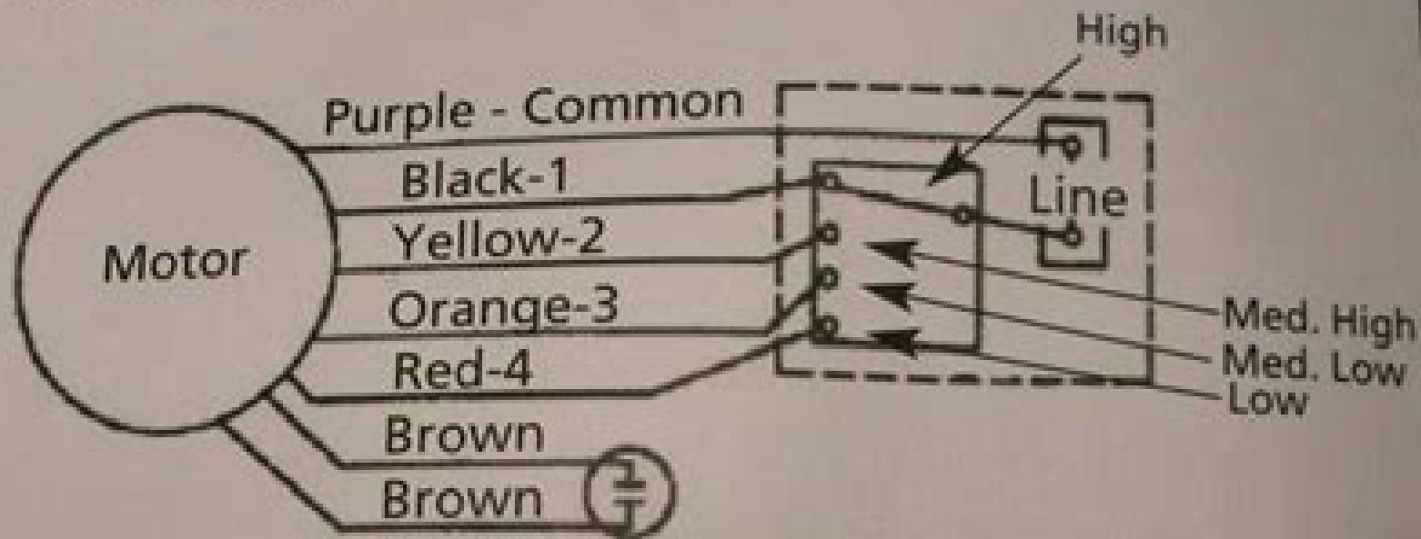
Figure 2 - Wiring Diagrams
