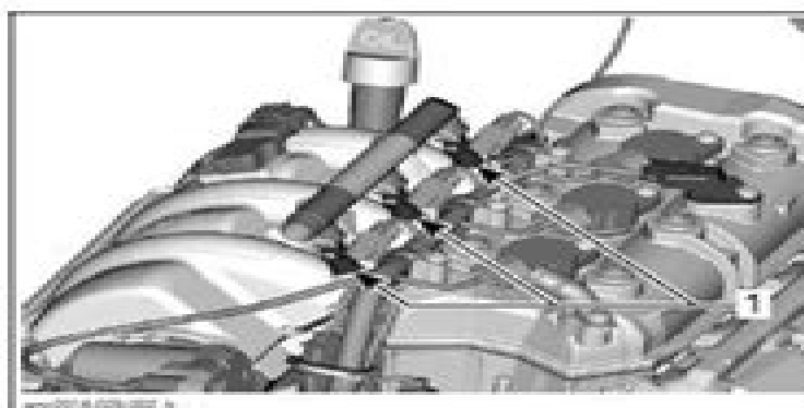
1. Fuel injectors
