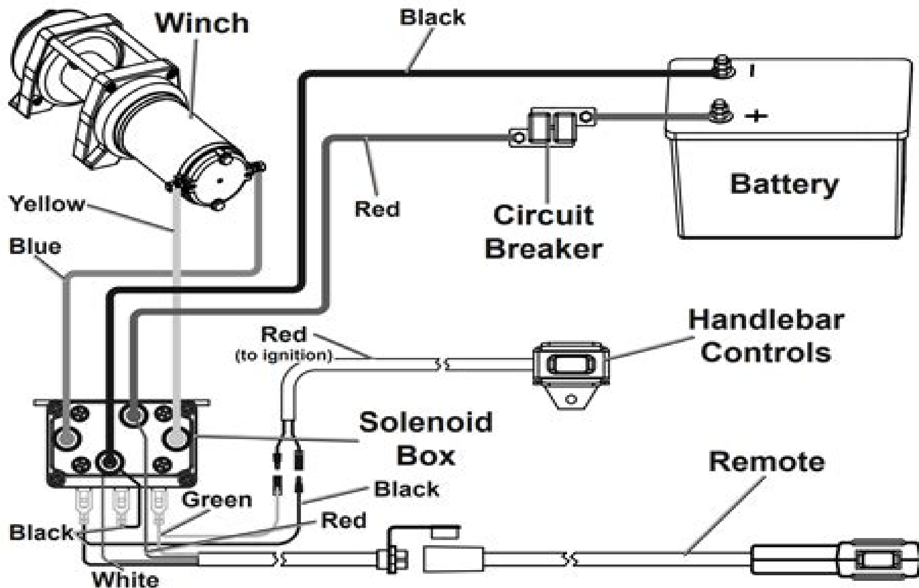
Figure E: Wiring Connections
