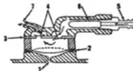
Fig. SK1-5—Schematic view of the diaphragm type fuel pump used on all models. Check valves are of the reed type.
