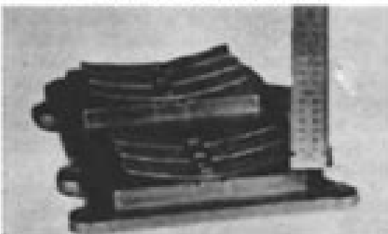
Fig. SK1-4—Reed stops should be 3/16-inch from seating surface of reed plate.
