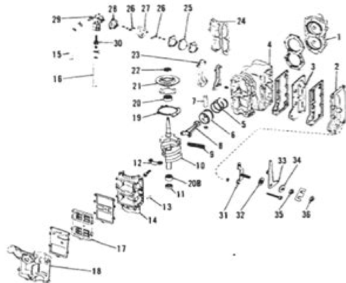
Fig. SK1-7—Exploded view of power head and associated parts. Bearing (208) is used on 8.2
