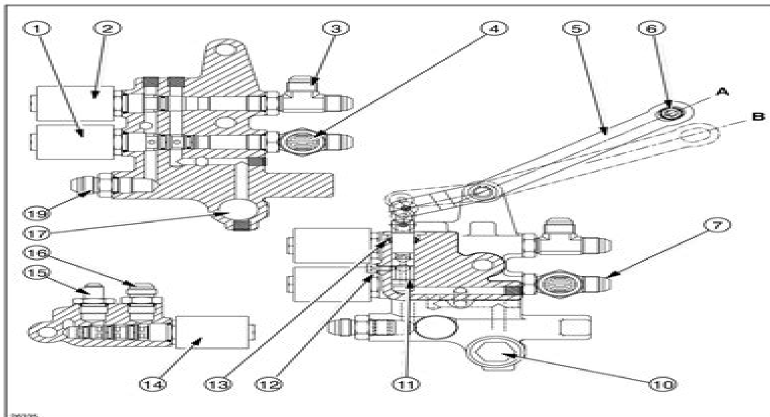
Sectional views of the services control valve with solenoid valves [tractor with Dual Command (2 Speed Power Shift)]
