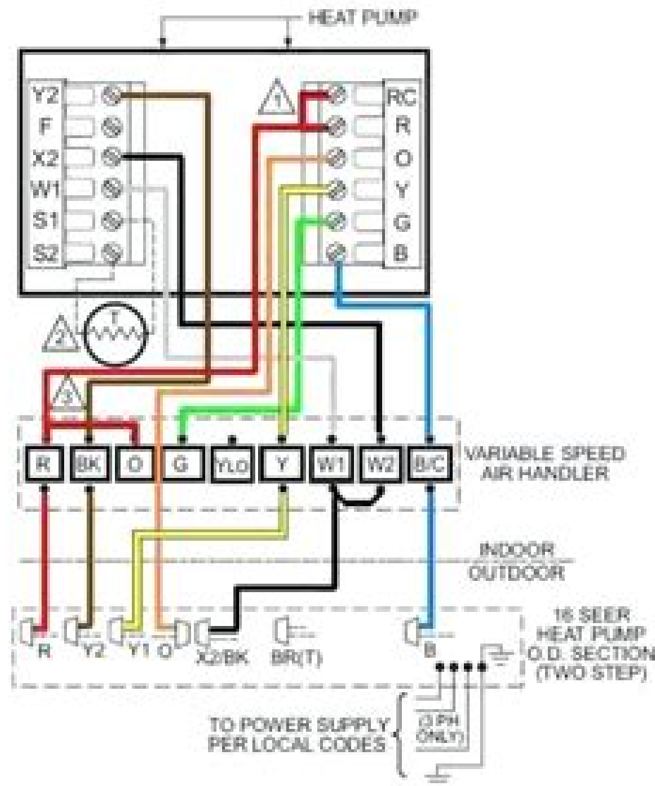
Fig. 11. Typical hookup of multistage two-step scroll heat pump with auxiliary/backup heat (3H/2C heat pump).
