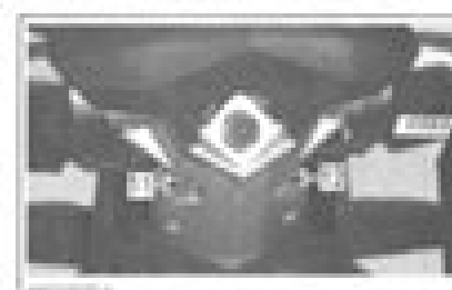
Image 2: Check engagement of cover housing steering and throttle
