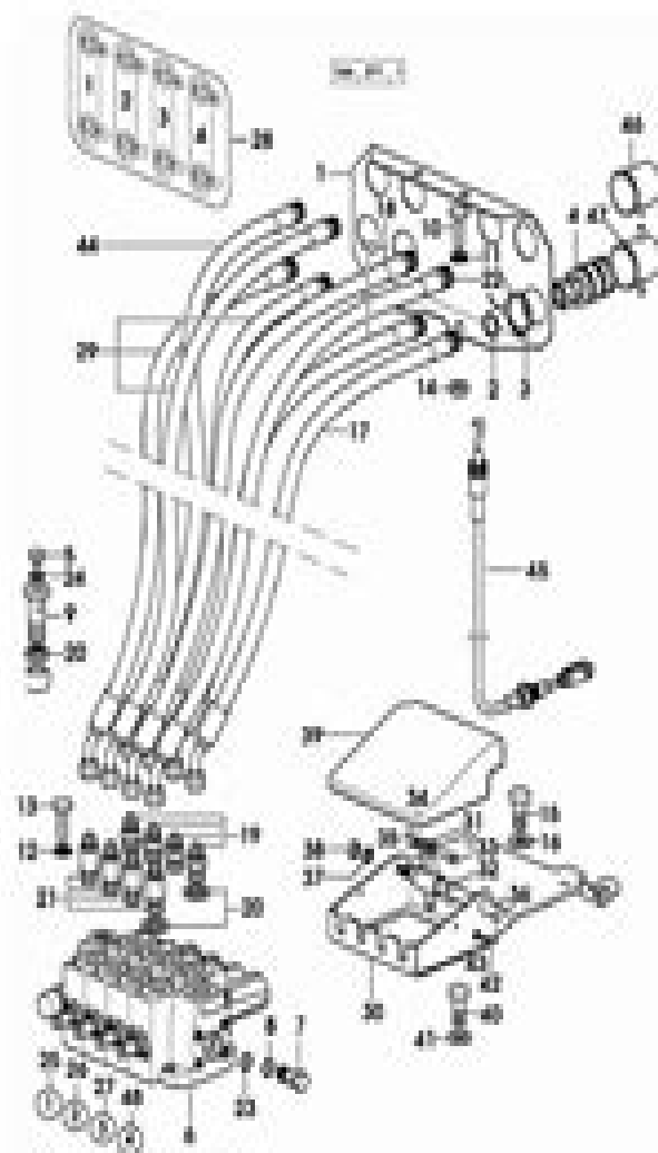
SILVER 110 Section: ACCESSORIES REXROTH SILVER 110 6-WAY AUXILIARY CONTROL VALVE Ref.: 06.00.4
