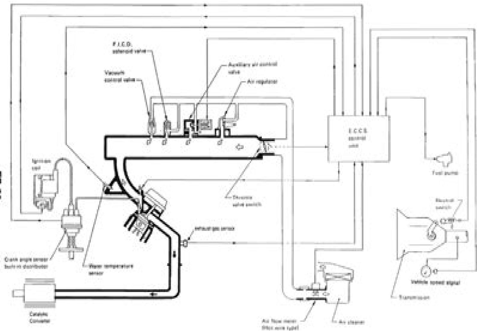
E.C.C.S. DIAGRAM
