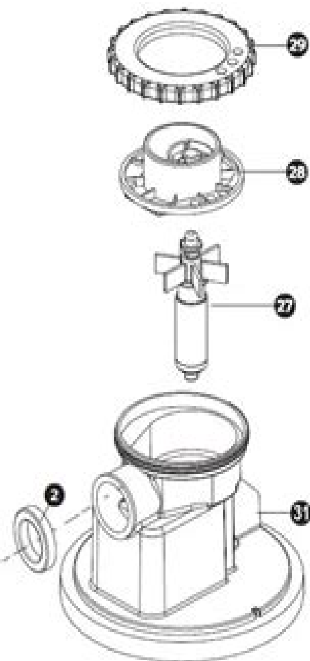
SFX600/SFX1000
