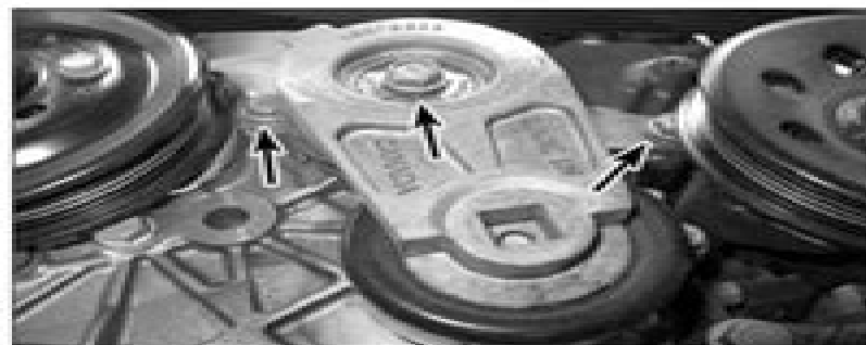
24.25 Typical V6 tensioner mounting fastener locations
