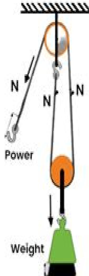
Compound Pulley
