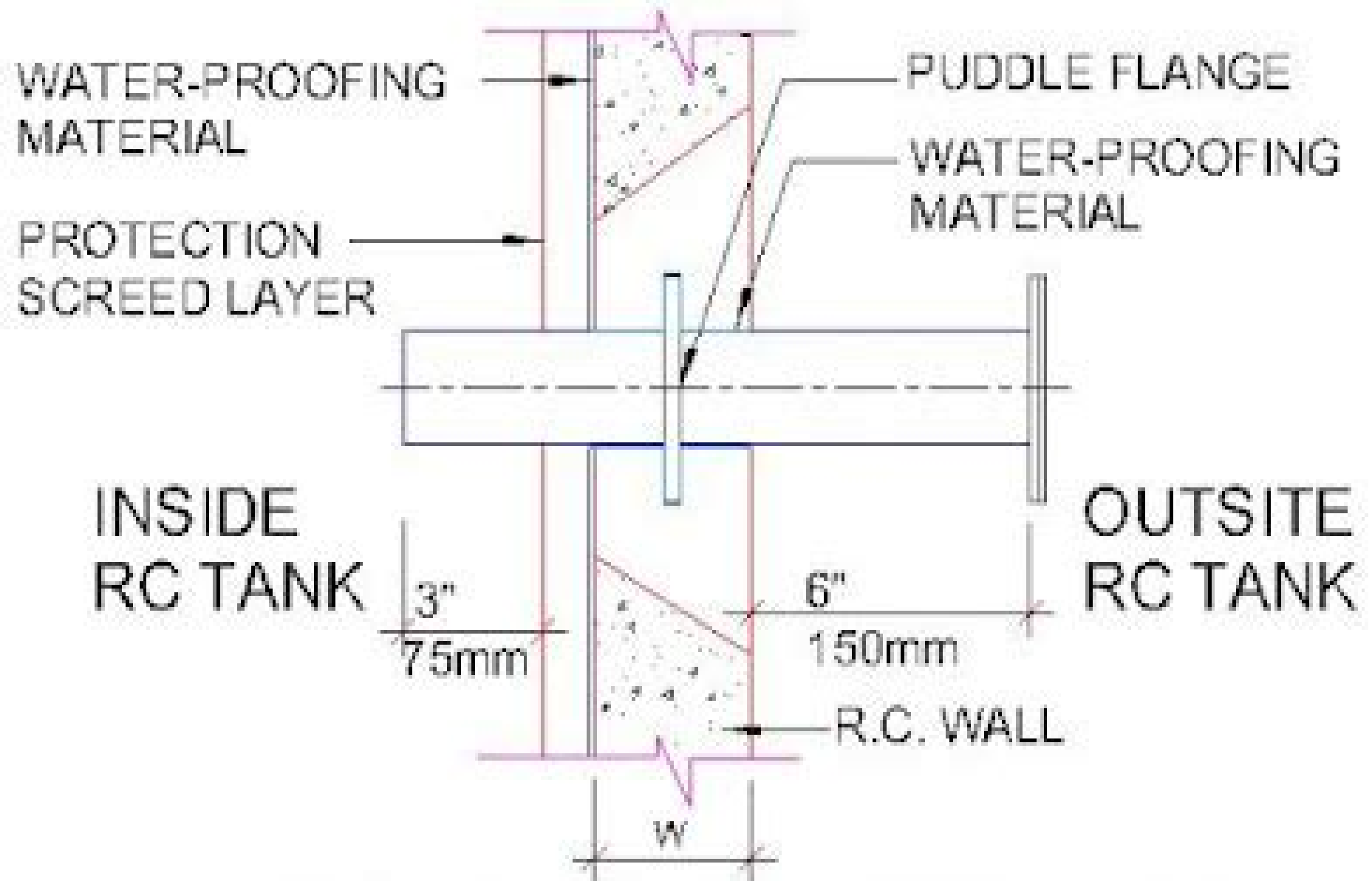
PUDDLE FLANGE INSTALLATION (SIDE ELEVATION)
